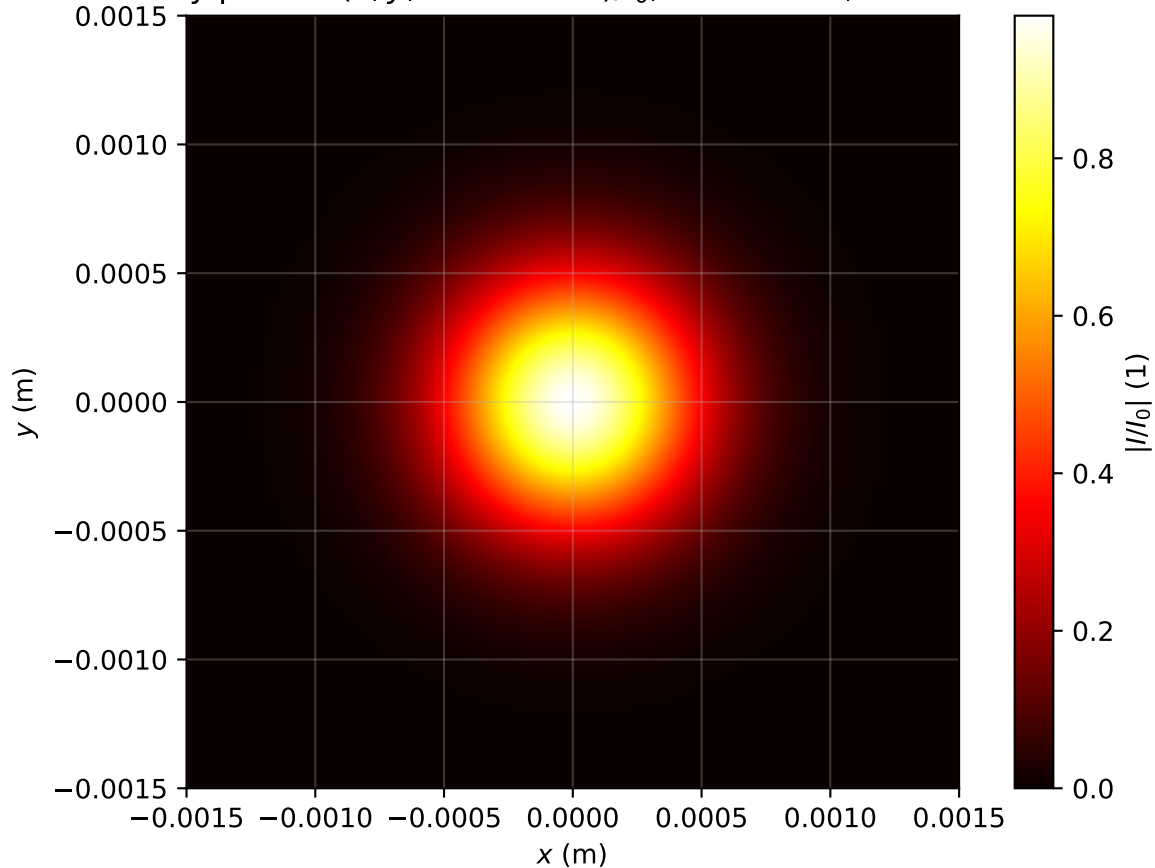
Intensity profile I(x, y, z = 0.478m)/I_0 , P_{in}=0.2P_{cr} , artificial time
